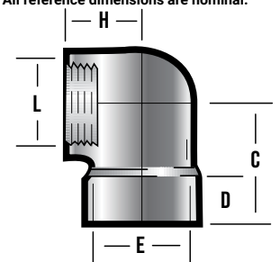
90° ADAPTER ELBOW
