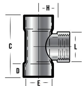
ADAPTER TEE
